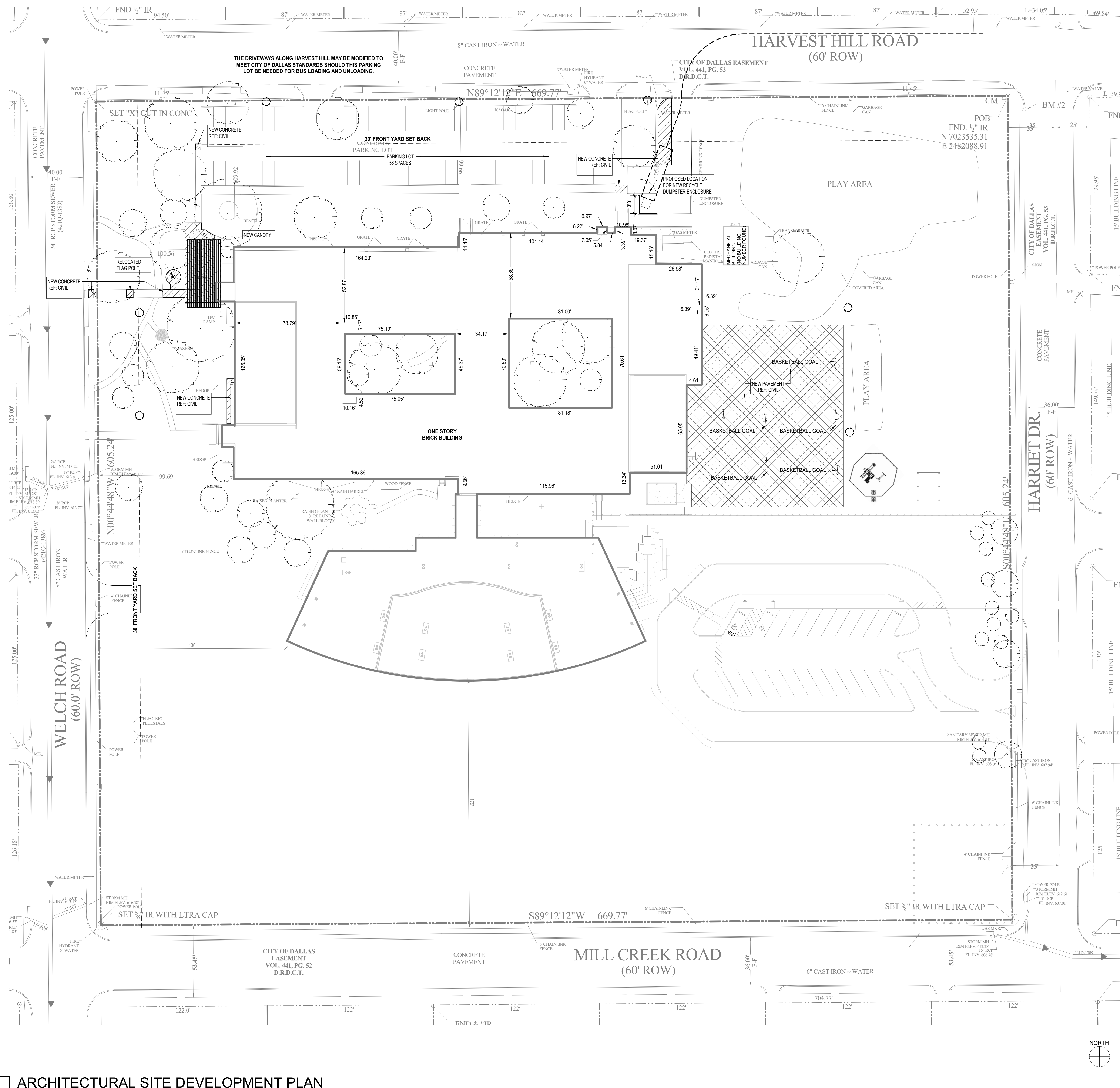
1 ARCHITECTURAL SITE DEVELOPMENT PLAN
